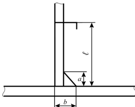
Figure 27: Bracket at lower end of ordinary stiffener on plane bulkhead
